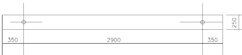
ITEM 8 3600 x 250 x 125 WOOD BAULK SCALE :- 1:20
