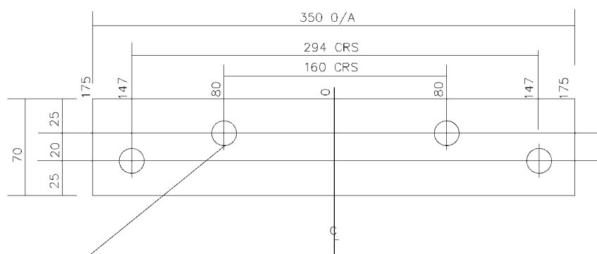
ITEM 10 70 x 15 x 350 LONG - FLAT BAR SCALE :- HALF FULL SIZE
